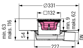
Rys.: Nr art. 44740.62M, 44750.62M, 44740.20M, 44750.20M
