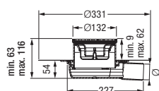
bez systemu Lock&Lift
